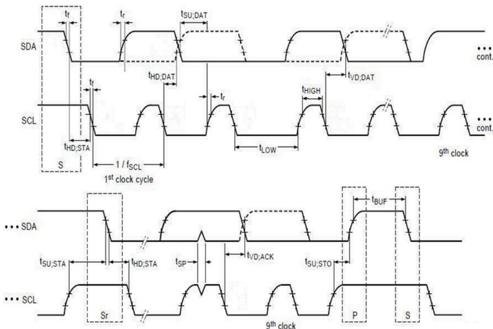
Figure 3: I2C peripheral specification
