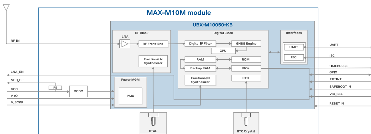
Figure 1: MAX-M10M block diagram
