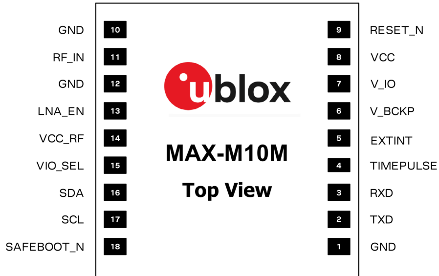
Figure 2: MAX-M10M pin assignment
